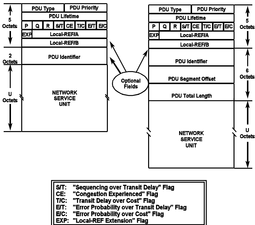
Figure 5.7-54 Compressed Initial and Derived PDU Formats
